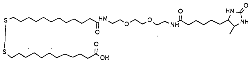
desthio compound 2
